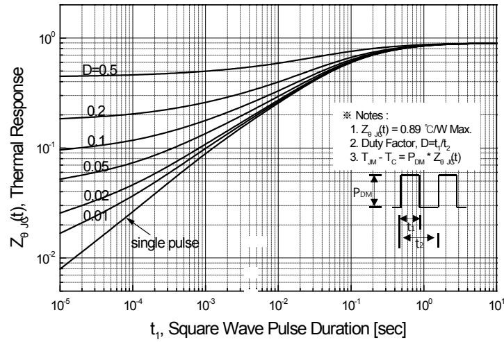
Figure 11-1. Transient Thermal Response Curve for SLP740C
