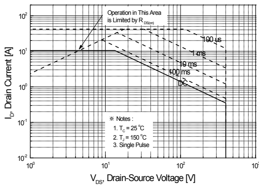
Figure 9-1. Maximum Safe Operating Area for SLP740C
