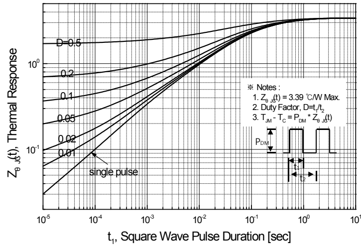
Figure 11-2. Transient Thermal Response Curve for SLF740C
