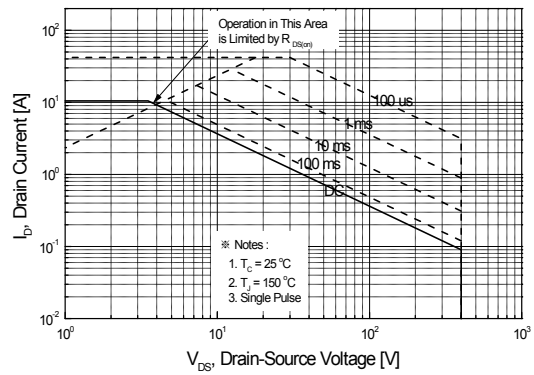
Figure 9-2. Maximum Safe Operating Area for SLF740C
